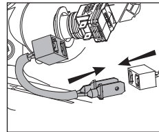
6 Use an additional connector cable if necessary
