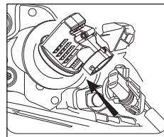
3 Connect the power cable with original car connector
